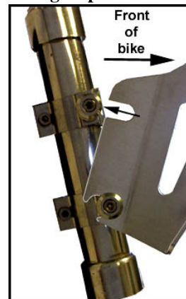
Fig. 3 plate to forks
