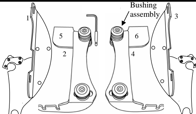
2321-0118 Fairing Mounting Kit
